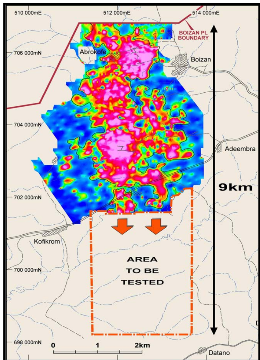
Boizan gold in soil anomaly (red greater than 50ppb gold) and untested southern extension
